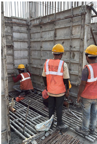
shuttering of the elevator wall
