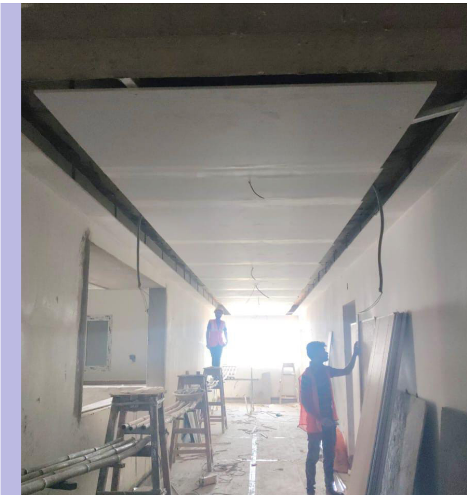
Installation of false ceiling in 3rd floor corridor.
